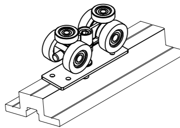
CH9591 Tommaslide roller assembly incl Bracket & Locknut 300kg
