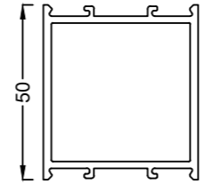
C4057EN M50 Midrail
