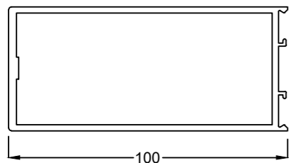
C056 Wide Plain Stile
