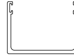
C3270 Door Channel 60 x 44.4mm
