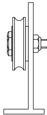
CH10 Top roller Assembly 250kg
