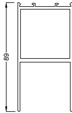
C052 Bottom Rail
